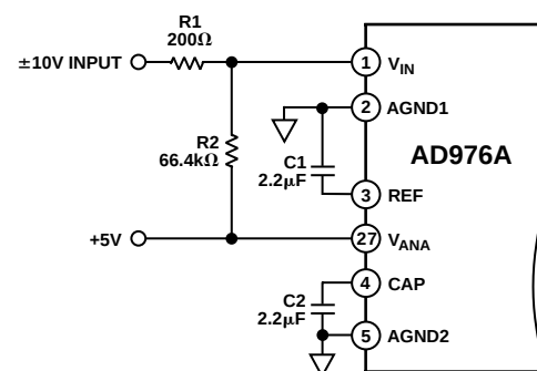
Figure 6. \pm 10 V Input Connection for the AD976A (Internal Reference) Only
