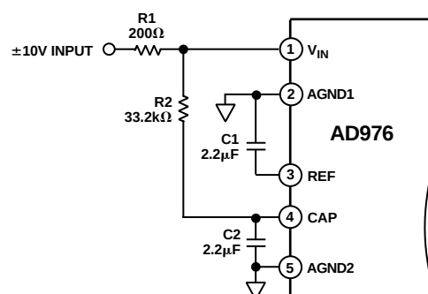
Figure 5. \pm 10 V Input Connection for the AD976 (Internal Reference)
