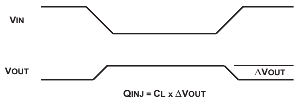
Figure 5. Charge Injection
