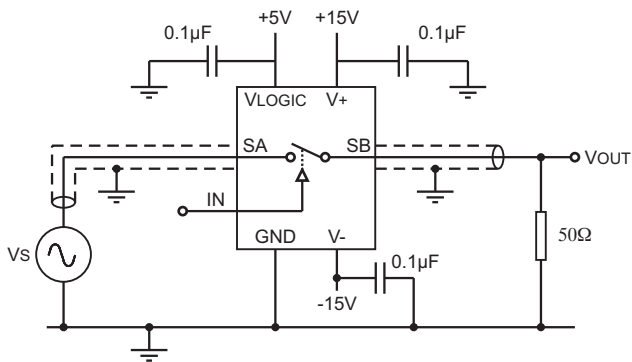
Figure 6 - Off Isolation
