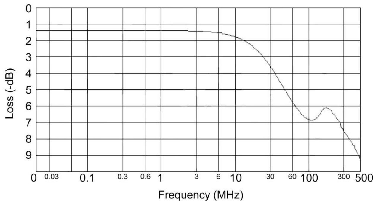
Figure 10. Frequency Response.
