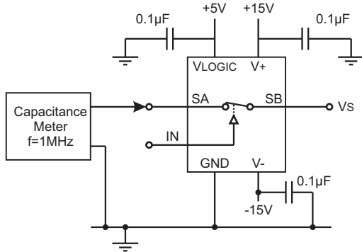
Figure 9 - On Capacitance
