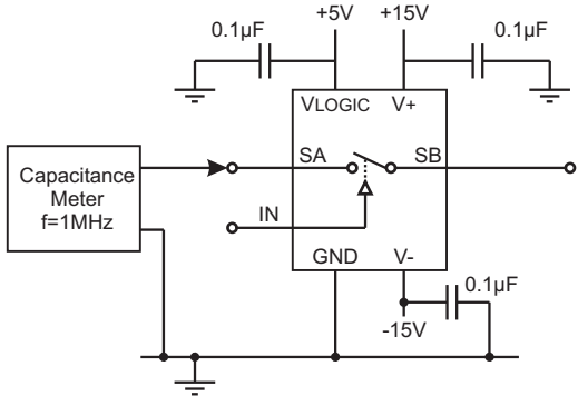
Figure 8 - Off Capacitance
