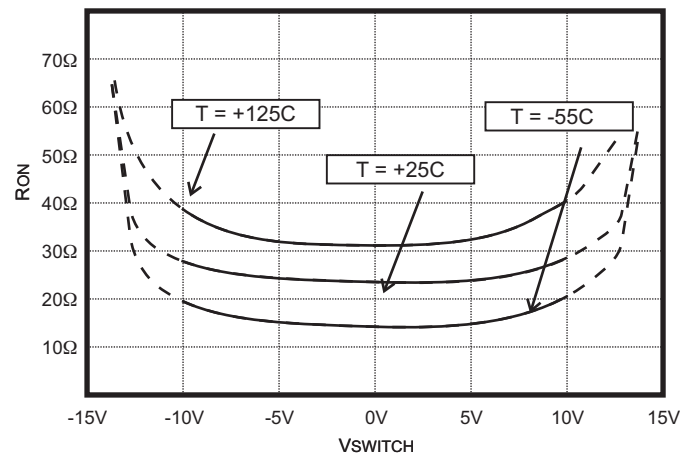
Typical RON as a function of VSWITCH and Temperature (10mA switch current, VSUPPLY = +/-15V)
