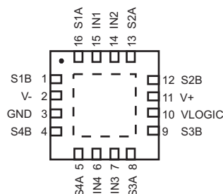
HI-8195PCx 16-pin 5mm x 5mm Chip-scale package
