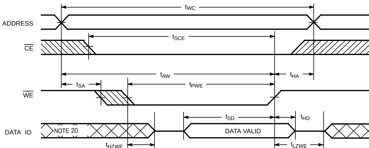
Figure 6. Write Cycle No. 3 ( \overline{\text{WE}} controlled, \overline{\text{OE}} LOW) [10, 19]
