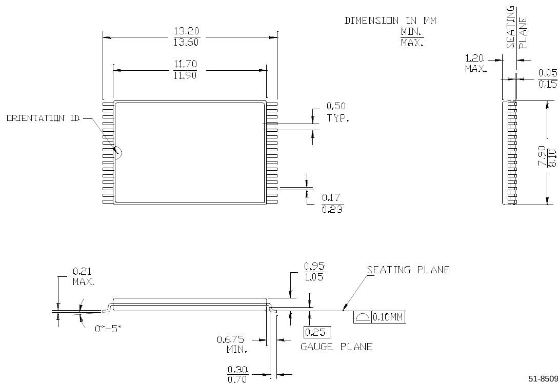
Figure 9. 32-Pin Shrunk Thin Small Outline Package (8 x 13.4 mm), 51-85094
