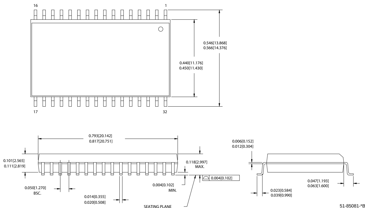
Figure 7. 32-Pin (450 Mil) Molded SOIC, 51-85081
