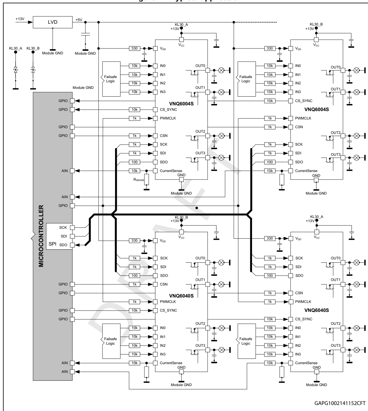
Figure 24. Typical application
