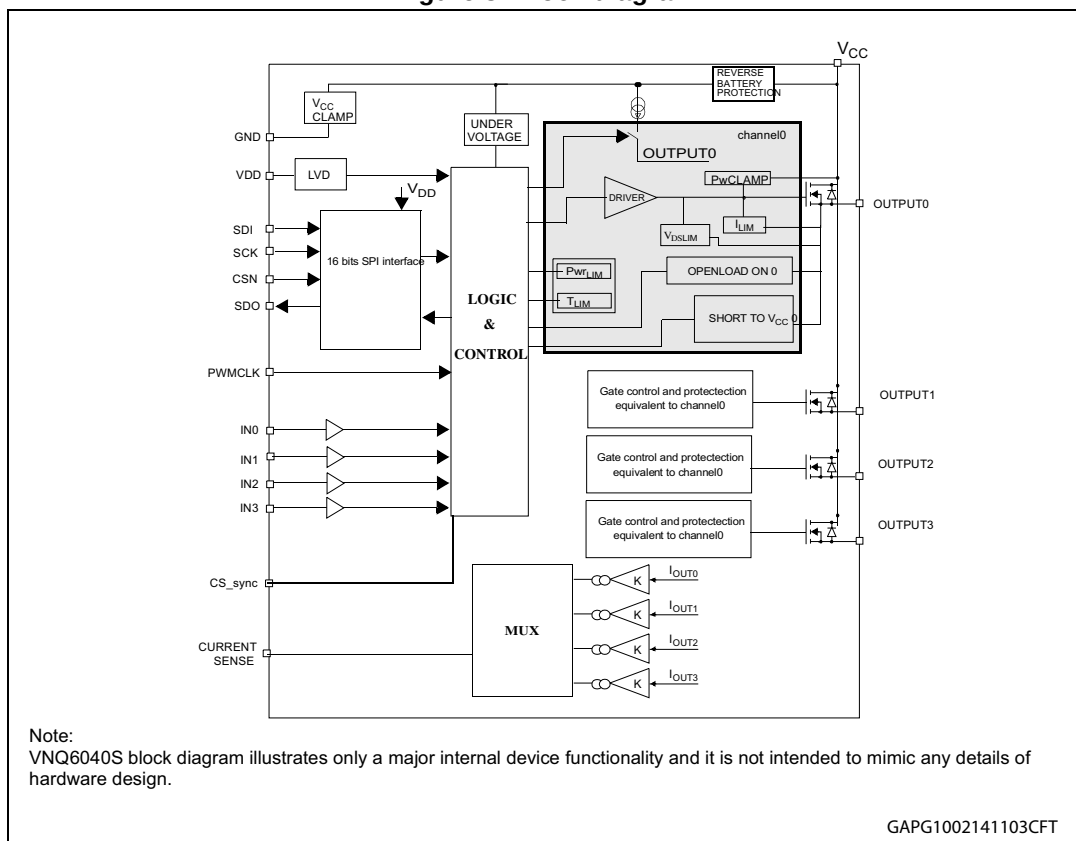
Figure 3. Block diagram
