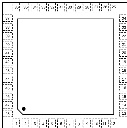
Figure 1. 48 WQFN Package (Top View) Package Number NJV0048A
