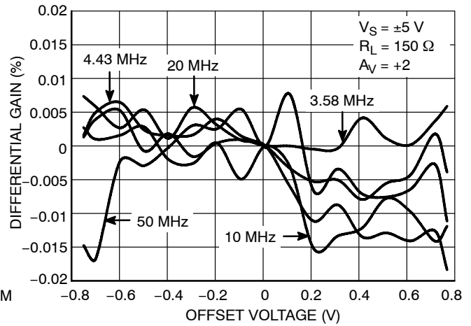
Figure 16. Differential Gain
