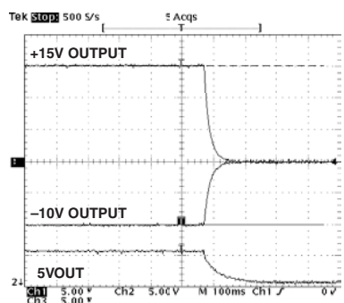
TPC 13. +15 V and -10 V Outputs at Power-Down (Unloaded)
