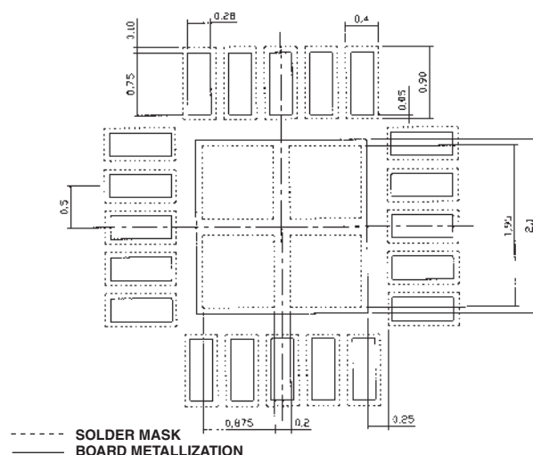
Figure 3. Suggested LFCSP 4 × 4 20-Lead Land Pattern
