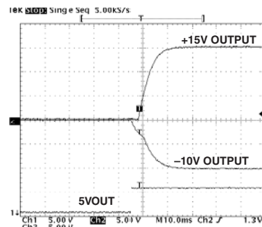
TPC 12. +15 V and -10 V Outputs at Power-Up
