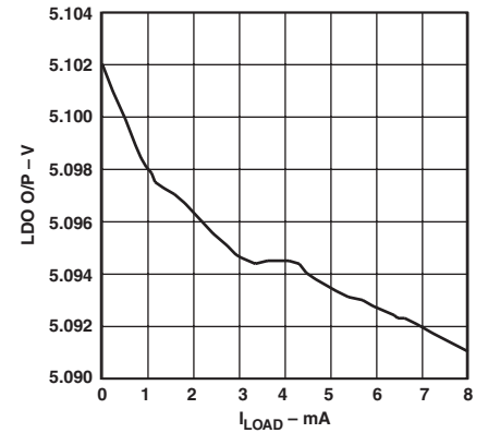
TPC 3. LDO O/P Voltage vs. Load Current in Scanning Mode, V_{CC} = 3.3\text{ V}
