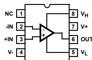
HFA1135 (SOIC) TOP VIEW
