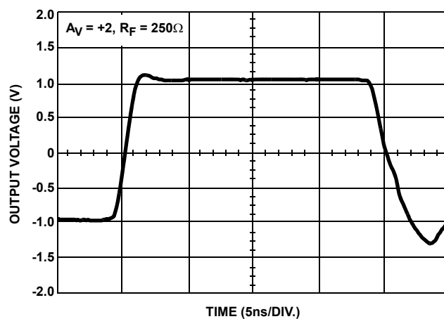
FIGURE 9. LARGE SIGNAL BIPOLAR PULSE RESPONSE
