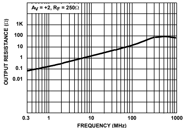
FIGURE 27. OUTPUT RESISTANCE
