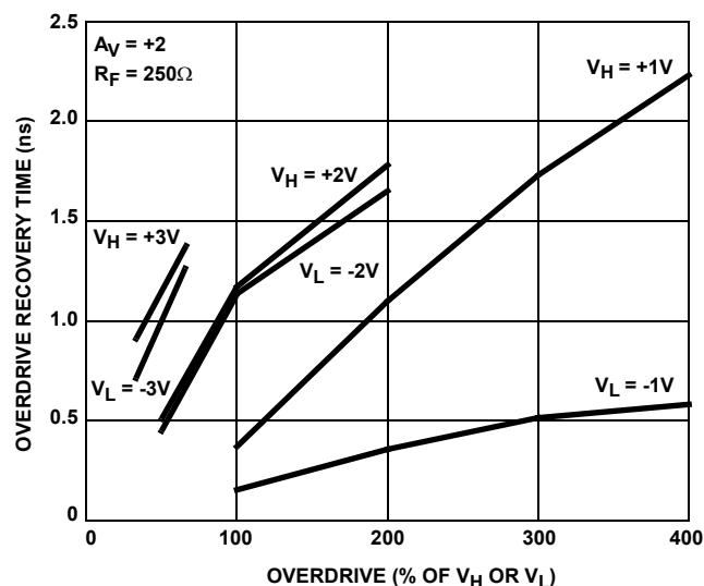
FIGURE 36. OVERDRIVE RECOVERY TIME vs OVERDRIVE
