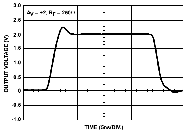
FIGURE 7. LARGE SIGNAL POSITIVE PULSE RESPONSE
