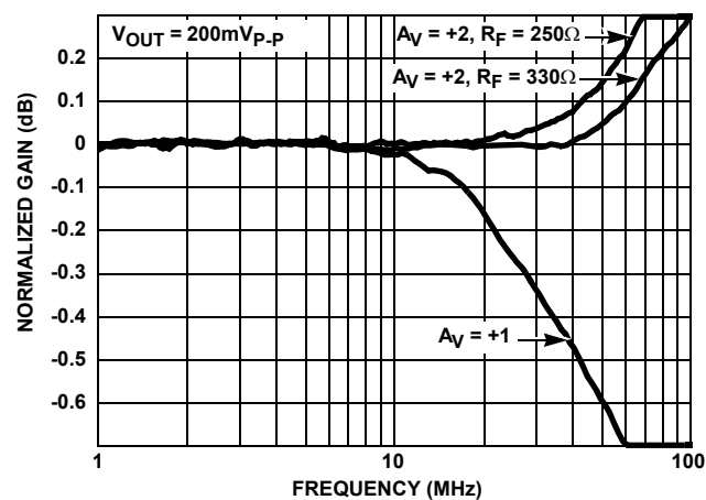
FIGURE 24. GAIN FLATNESS
