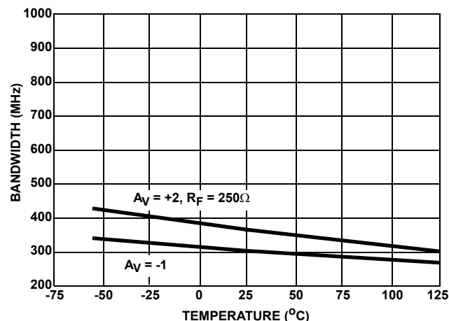
FIGURE 23. -3dB BANDWIDTH vs TEMPERATURE
