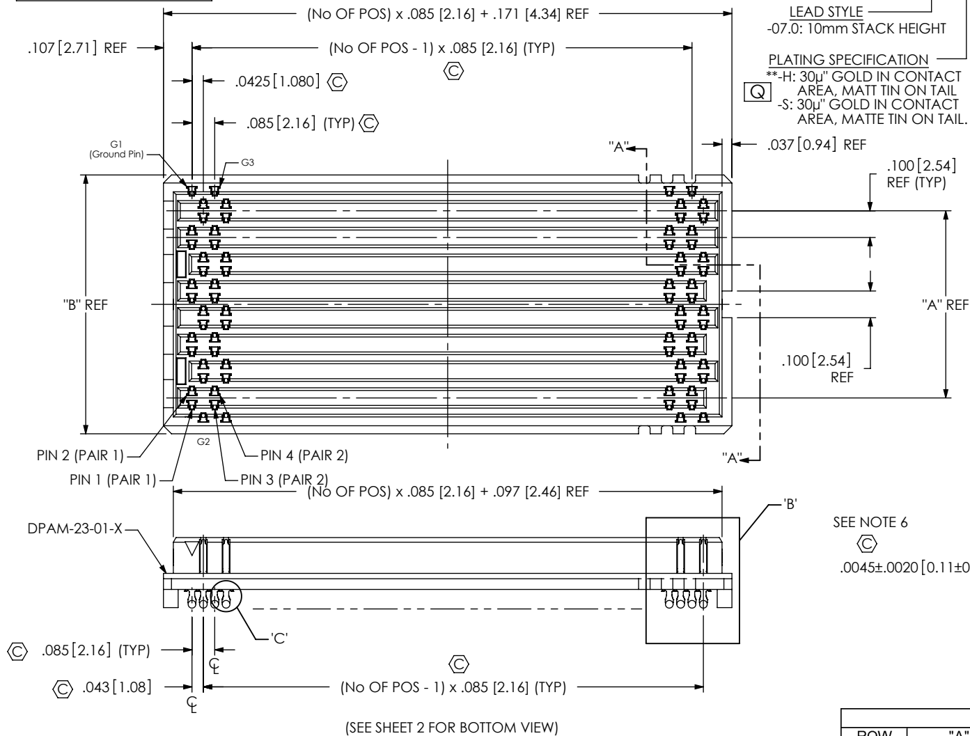
FIG 1 DPAM-23-07.0-X-8-1 SHOWN (ALL TERMINALS NOT SHOWN FOR CLARITY)
