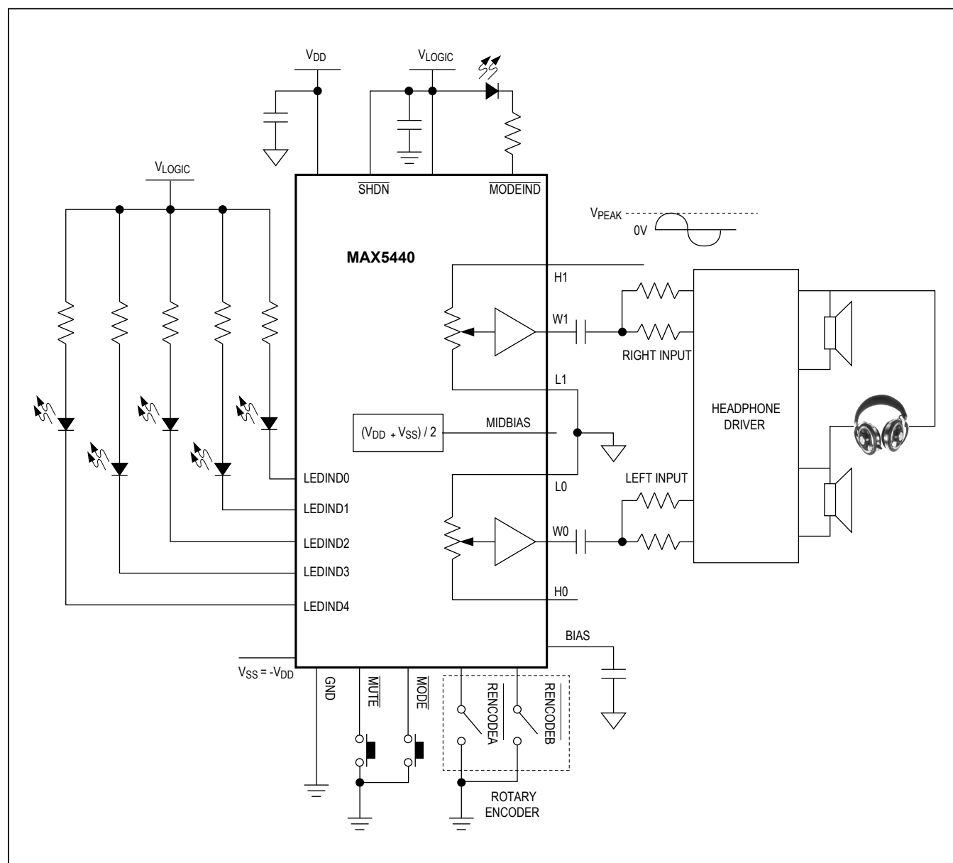
Figure 6. Dual-Supply Volume/Balance Control
