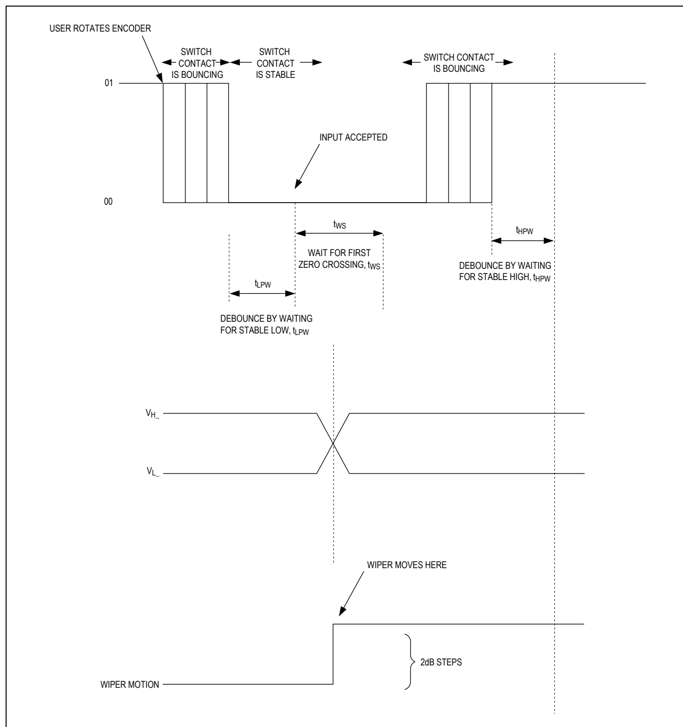
Figure 4a. Wiper Transition Timing Diagram—Suppression Circuitry Active
