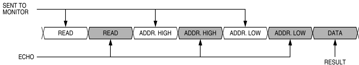
Figure 14-4. Read Transaction
