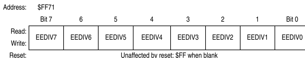
Figure 7-8. EEPROM-2 Divider Nonvolatile Register Low (EE2DIVLNVR)
