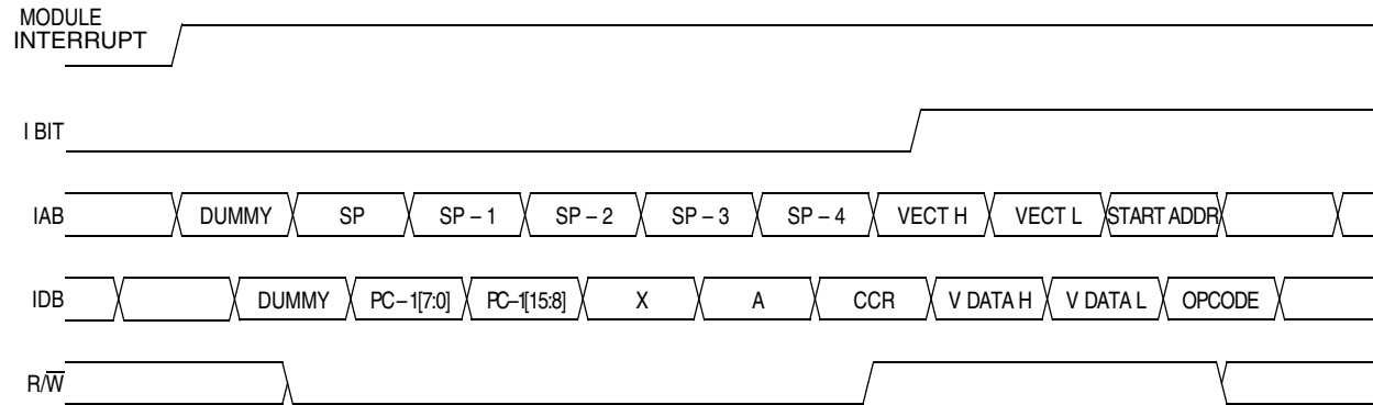
Figure 9-8. Interrupt Entry
