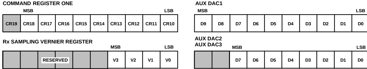
Figure 7. Internal AD7013 Registers
