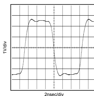
Fig.44 Output Waveform (VDD=5.0V, Select="L", Output=75MHz)
