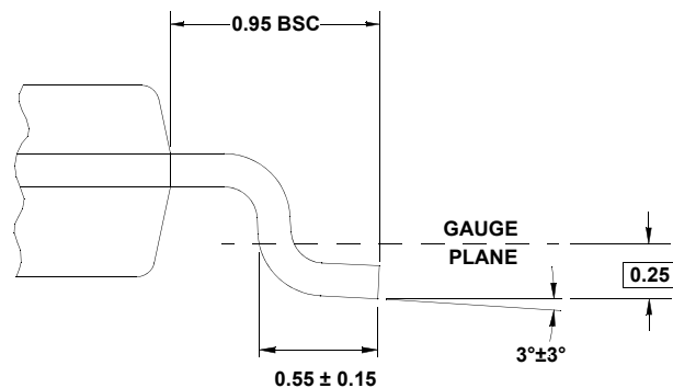
DETAIL "X"
