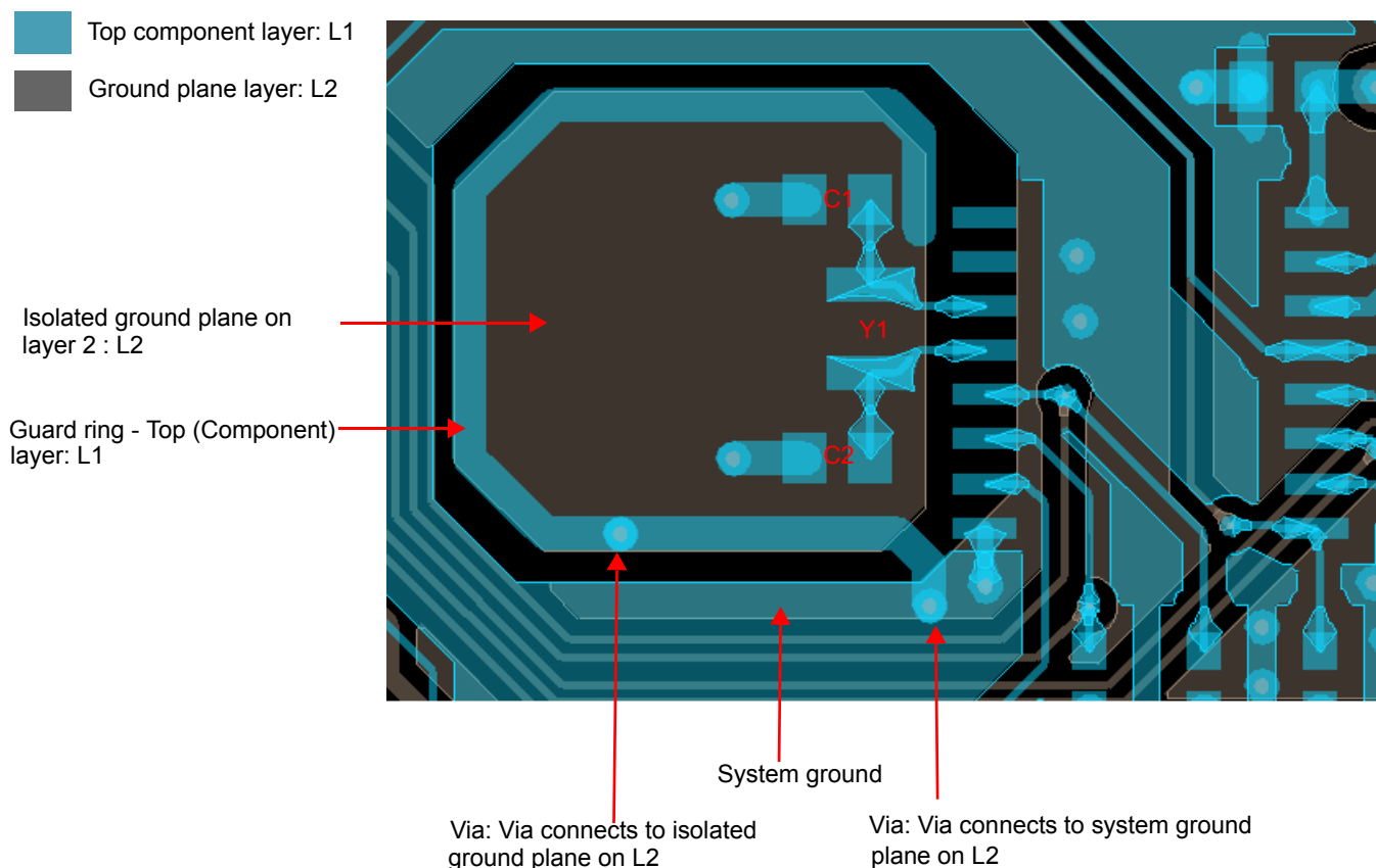
Figure 39. Recommended Layout for RTC
