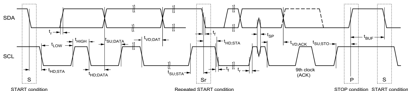
Figure 41. Timing Diagram
