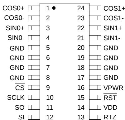
Figure 3. 33970 Pin Connections
