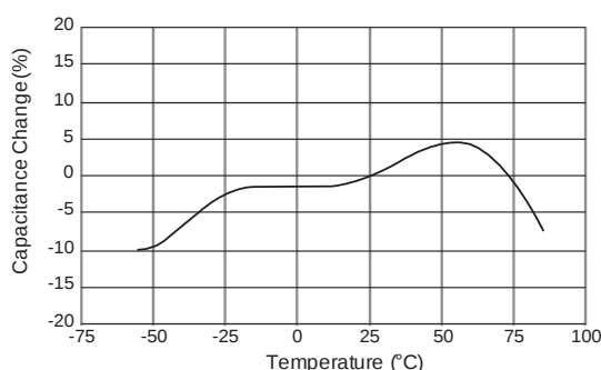
[Example of Temperature Characteristics R6] Sample: 22 \mu F, Rated Voltage 4VDC
