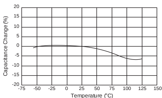
[Example of Temperature Characteristics R7] Sample: 0.1 \mu F, Rated Voltage 50VDC
