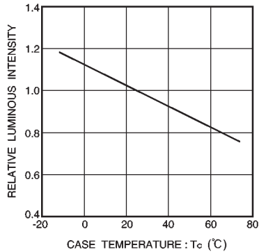
Fig. 23 Luminous intensity vs. case temperature
