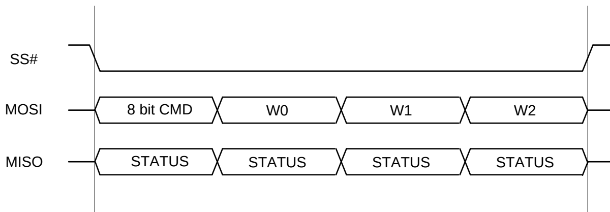
Figure 6.8 Half Duplex Data Master Write
