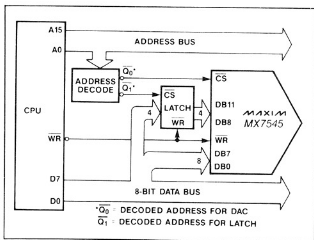
Figure 9. 8-Bit Processor to MX7545 Interface
