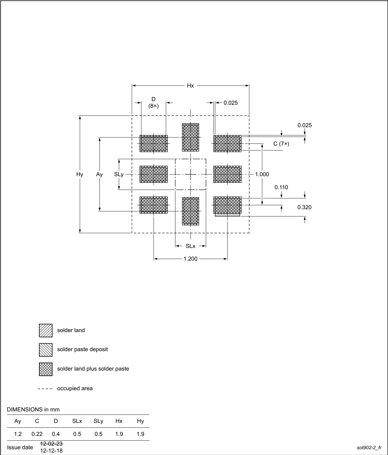
Fig 25. PCB footprint for SOT902-2 (XQFN8); reflow soldering
