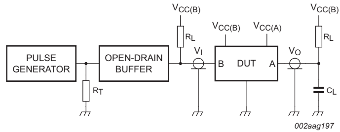
Fig 19. Test circuit for open-drain outputs A to B
