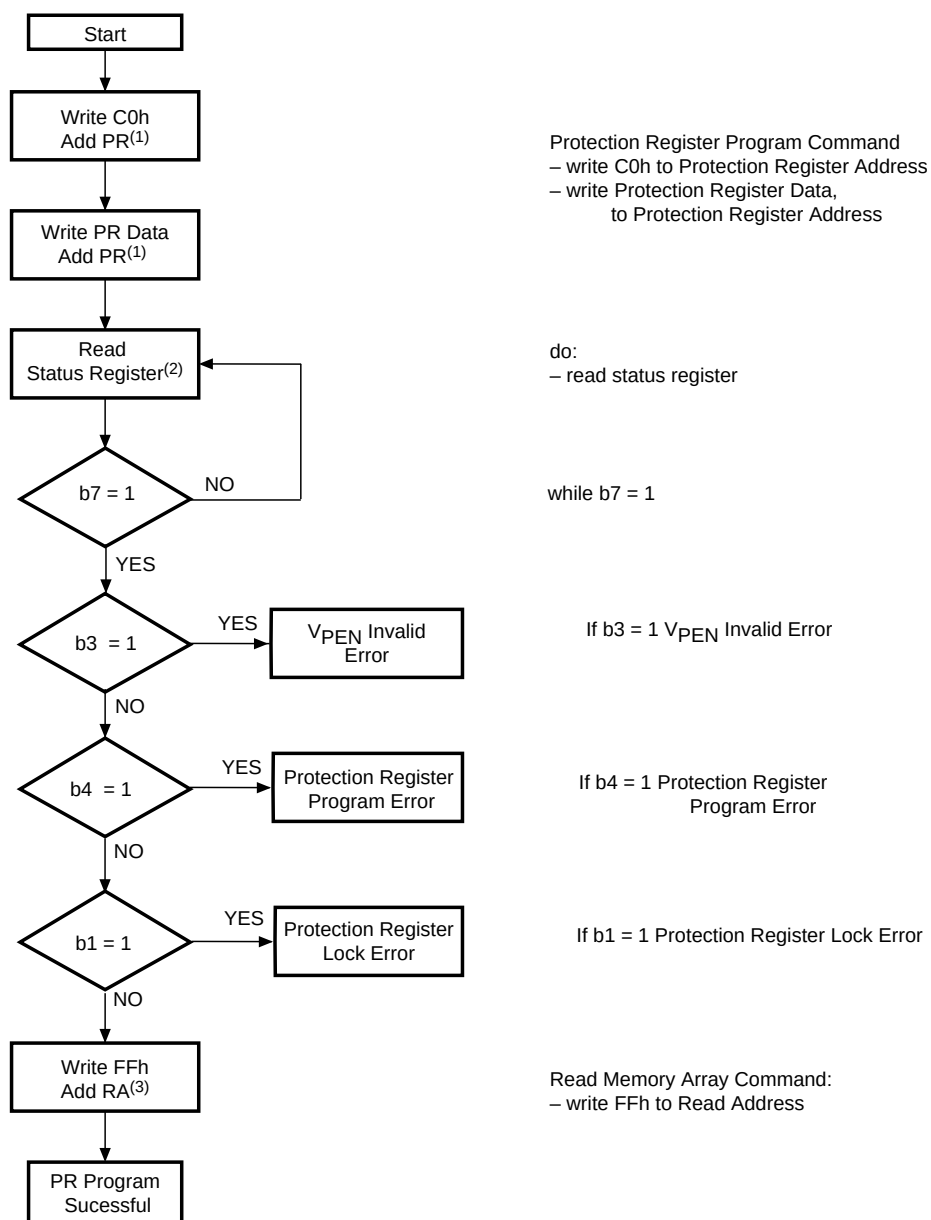
Figure 25. Protection Register Program Flowchart and Pseudo Code
