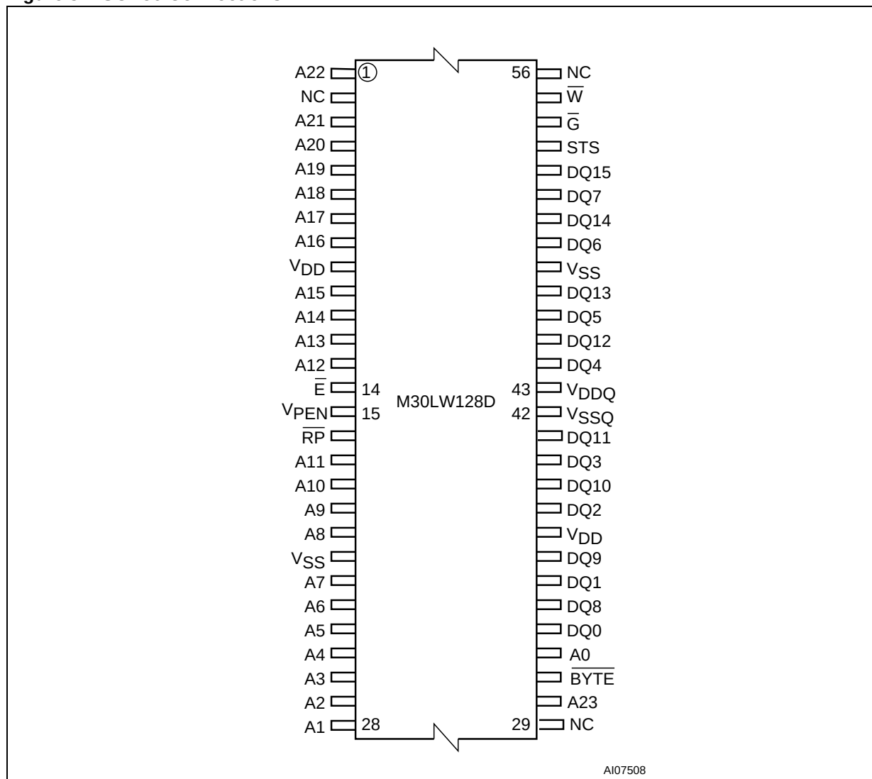
Figure 3. TSOP56 Connections
