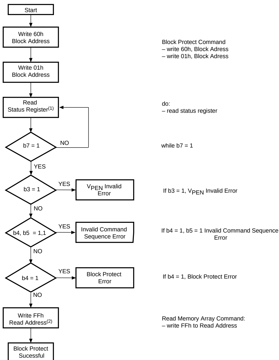
Figure 23. Block Protect Flowchart and Pseudo Code
