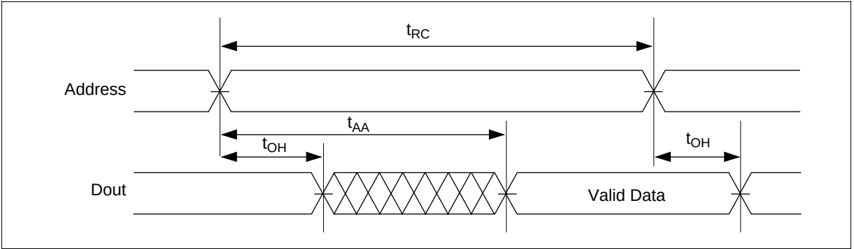
Read Timing Waveform (2)*1 ( \overline{WE} = V_{IH} )
