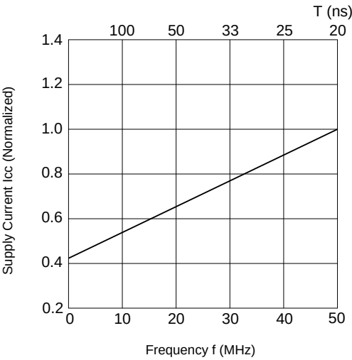
Supply Current vs. Frequency
