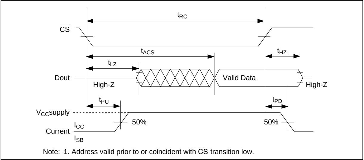
Read Timing Waveform (2)*1 ( \overline{WE} = V_{IH} )
