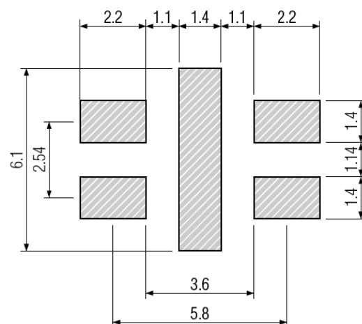
Figure 2) Land Pattern
