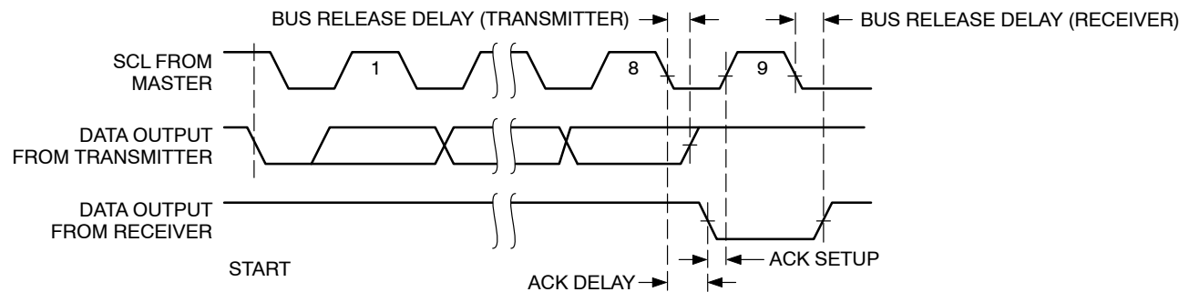
Figure 8. Acknowledge Timing
