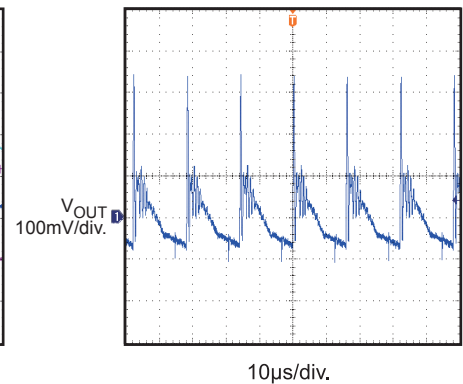
Output Ripple
