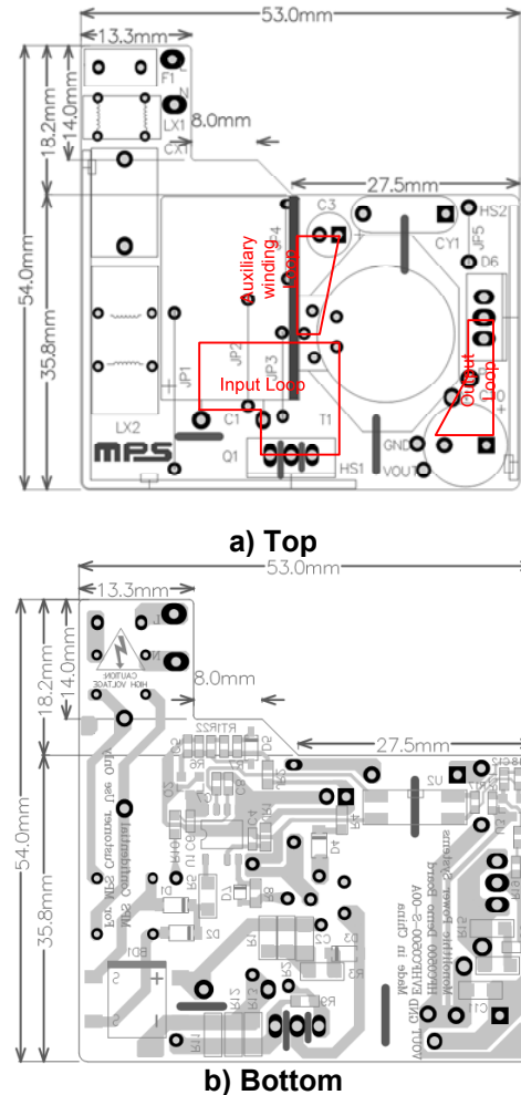
Figure 16: PCB Layout
