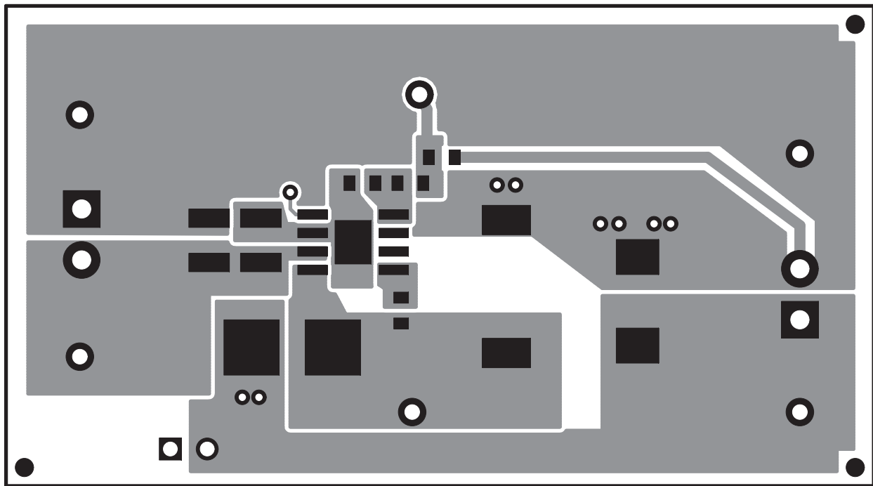
Figure 7. Top-side Layout
