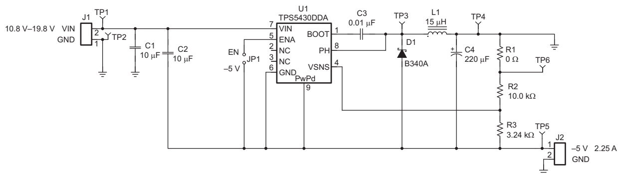
Figure 10. TPS5430EVM-342 Schematic
