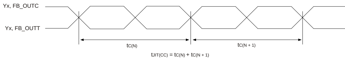
Figure 3: Cycle-to-Cycle Jitter
