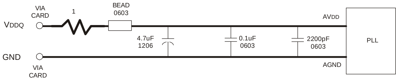
Figure 11. AVDD Filtering
