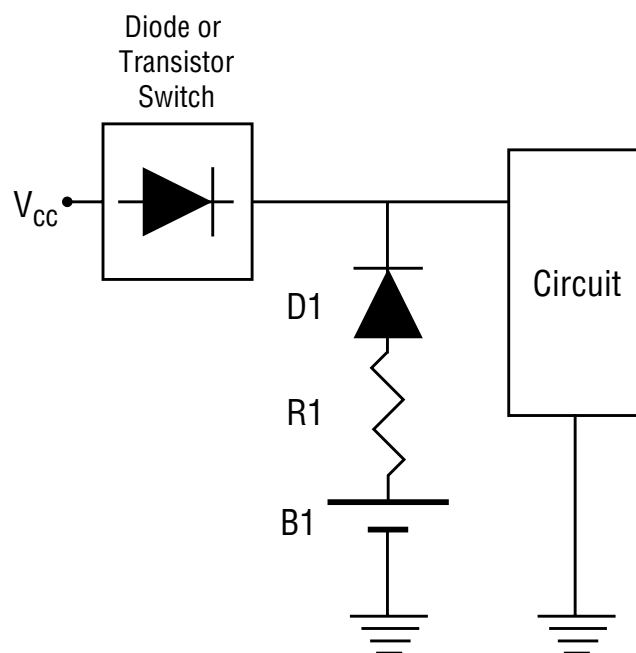
Protective Diodes and Limiting Resistor
