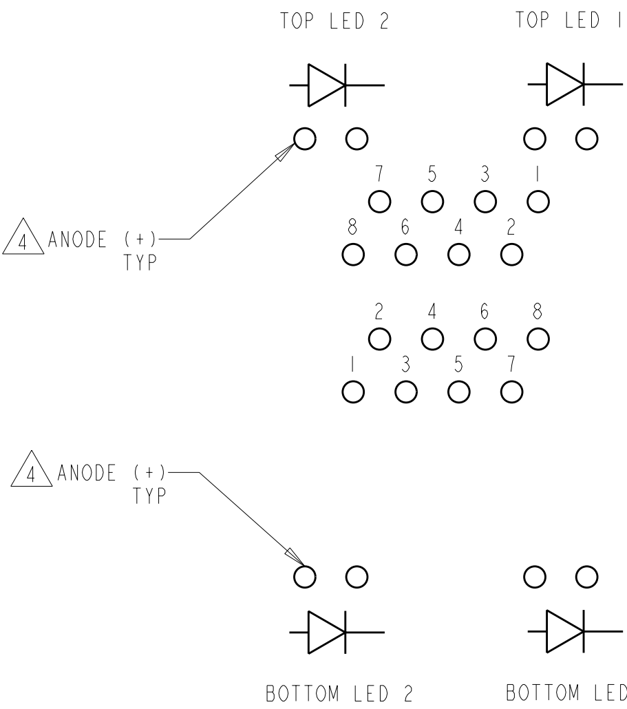
SCHEMATIC FOR 6116314-1, -2, -3 & -13 SCALE 4:1
