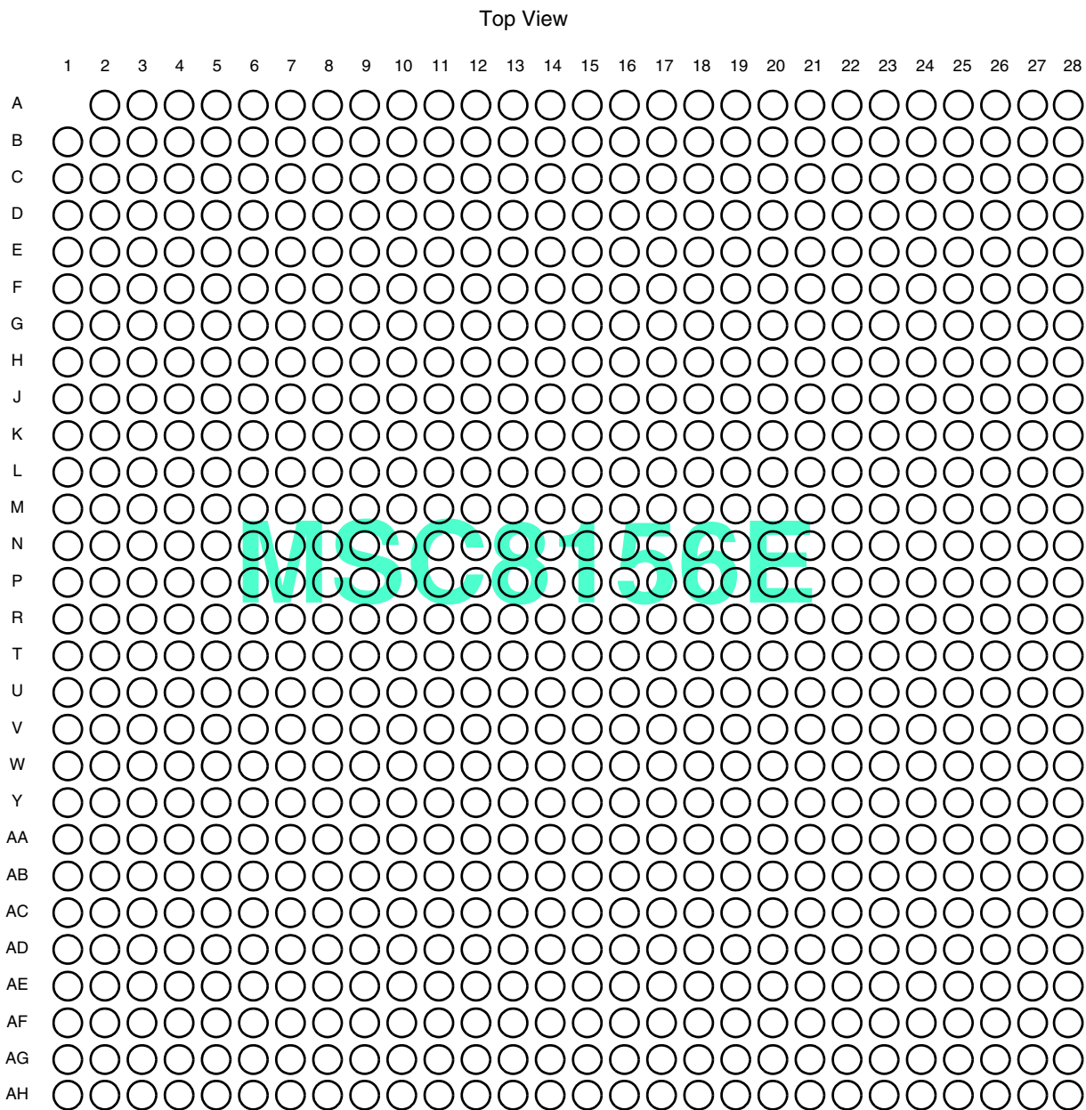
Figure 3. MSC8156E FC-PBGA Package, Top View
