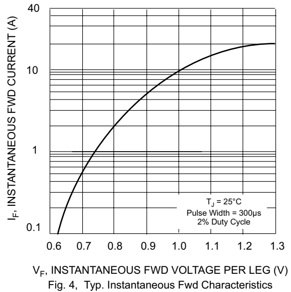
Fig. 4, Typ. Instantaneous Fwd Characteristics
