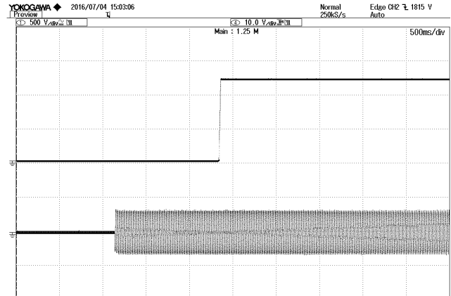
Figure 5: Vout start up with Enable on at 220Vac, 12A Iout, TOP: Vout, 10V/div, 500ms/div BOTTOM: Vin, 500V/div, 500ms/div
