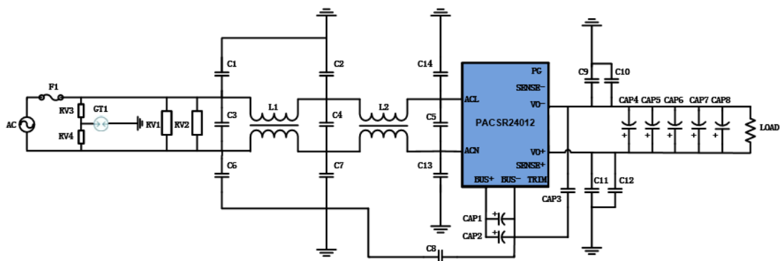
Figure 9: Application connection
