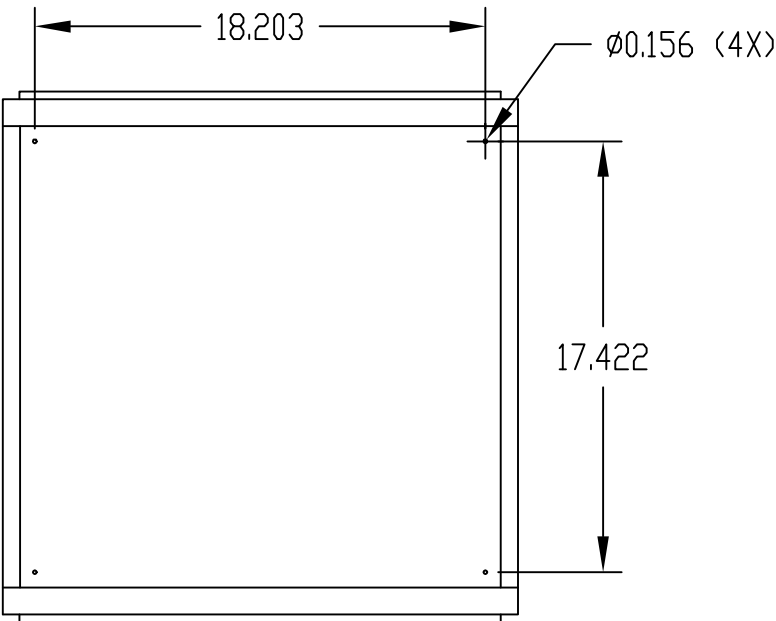
BOTTOM VIEW
