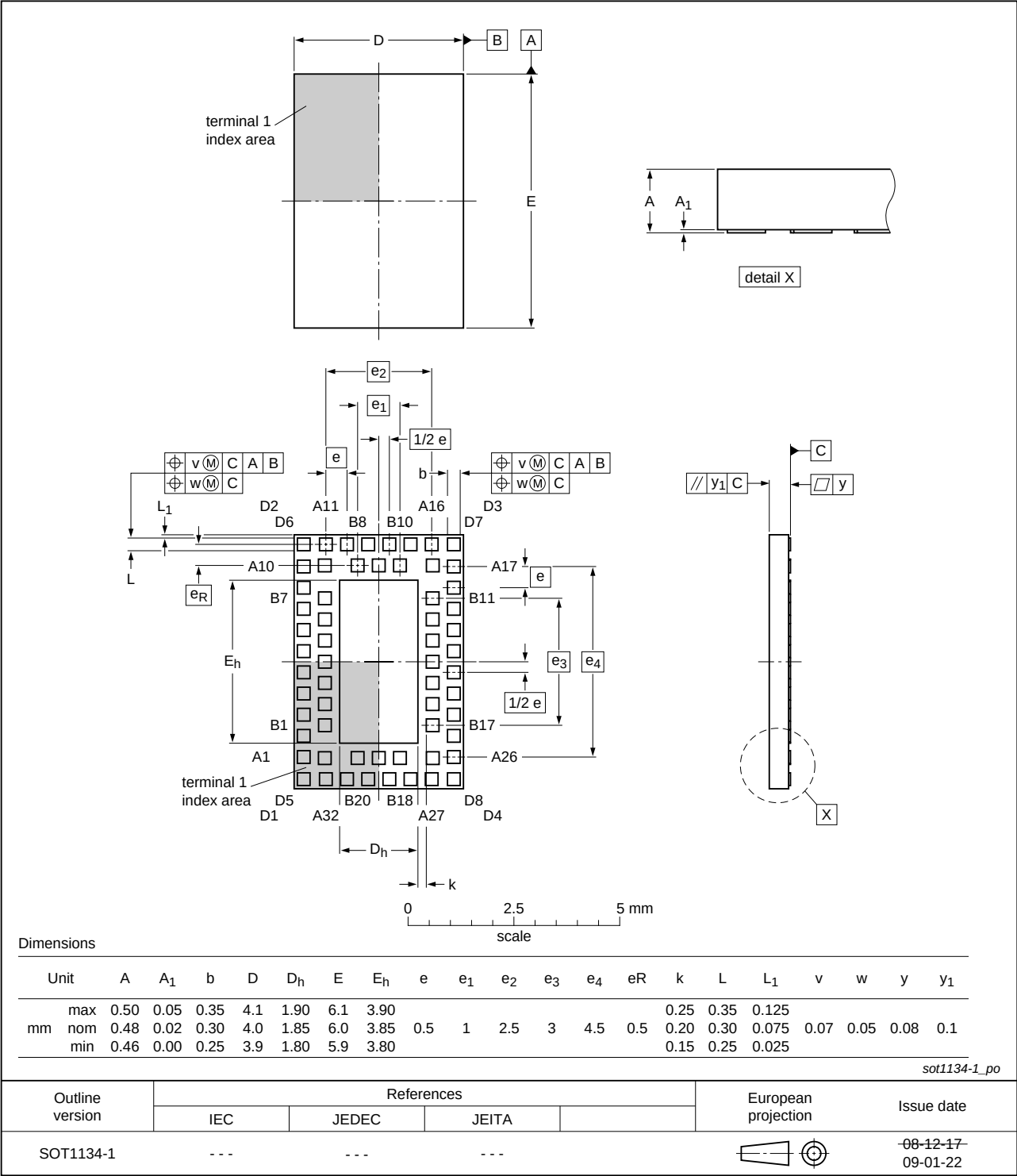
Fig 14. Package outline SOT1134-1 (HXQFN60U)
