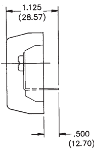
“Y” Terminals
