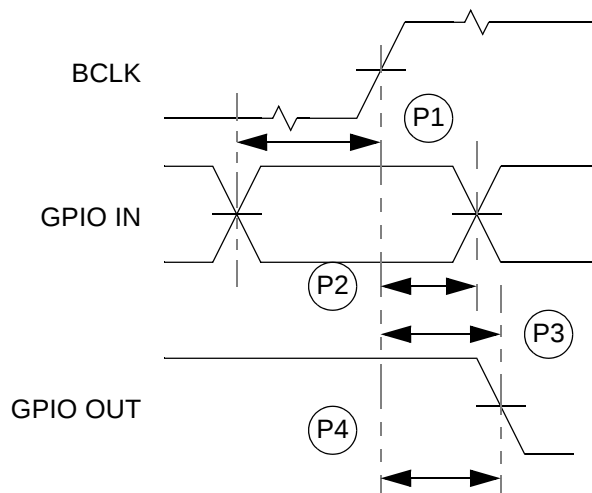
Figure 10. General-Purpose I/O Port AC Timing Definition Diagram
