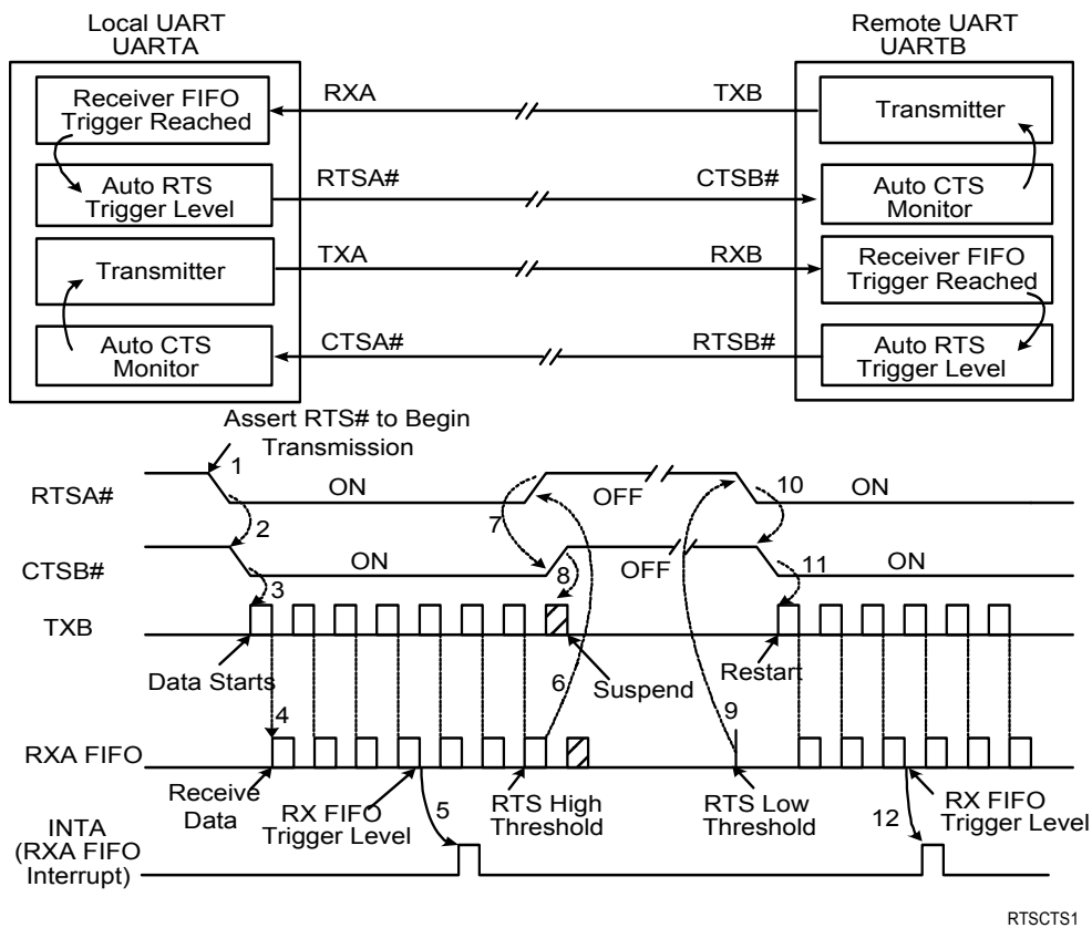
FIGURE 11. AUTO RTS AND CTS FLOW CONTROL OPERATION
