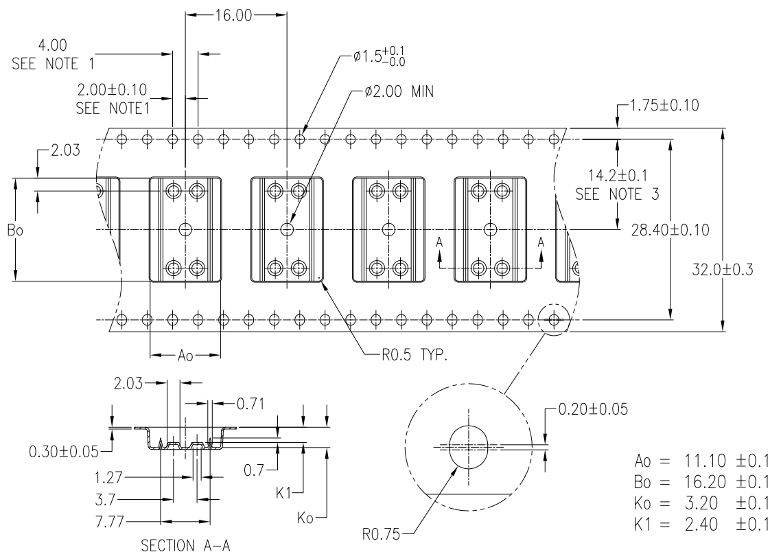
Figure 13. 48-pin SSOP (300 Mils) Carrier Tape, 51-51104
