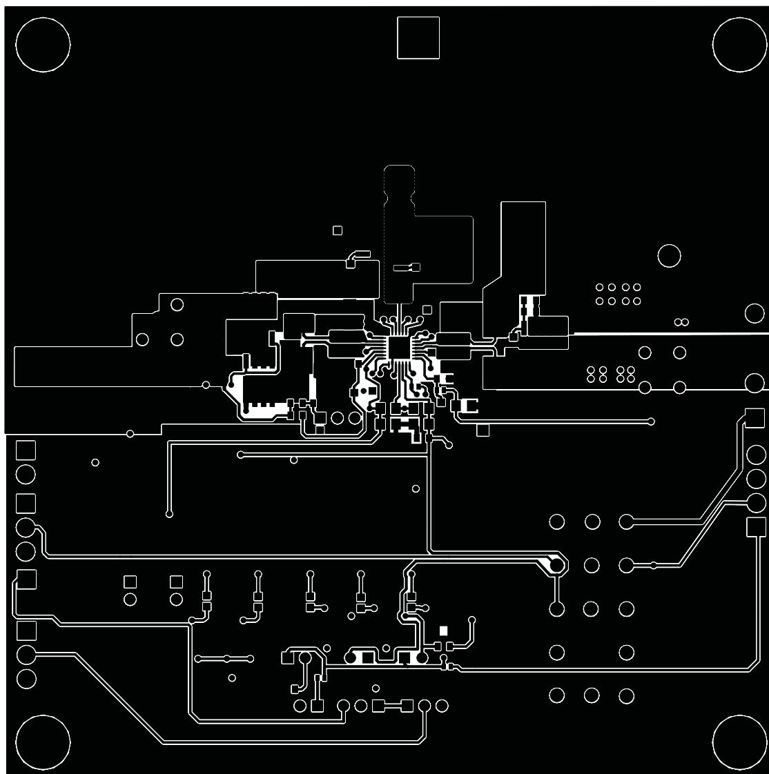
Figure 5. Top Layer
