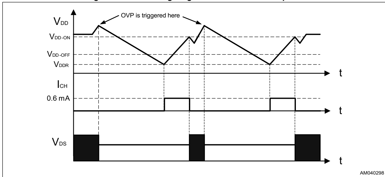
Figure 11. OVP timing diagram with auto-restart option
