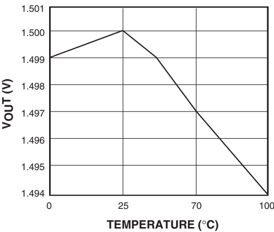
VOUT TEMPERATURE VARIATION
