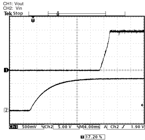
START-UP, 40A LOAD
