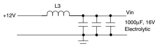
Figure 4. Input Filter
