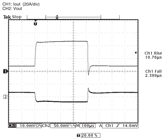
LOAD TRANSIENT, 12-52A
