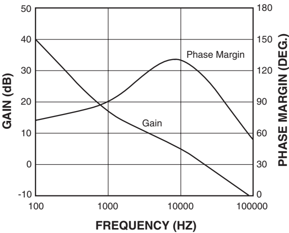
CLOSED LOOP RESPONSE, 40A LOAD
