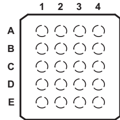
GQN OR ZQN PACKAGE (TOP VIEW)
