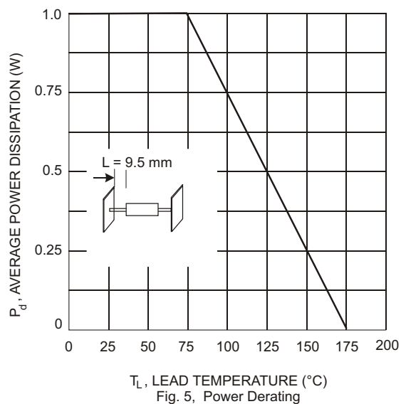
Fig. 5, Power Derating
