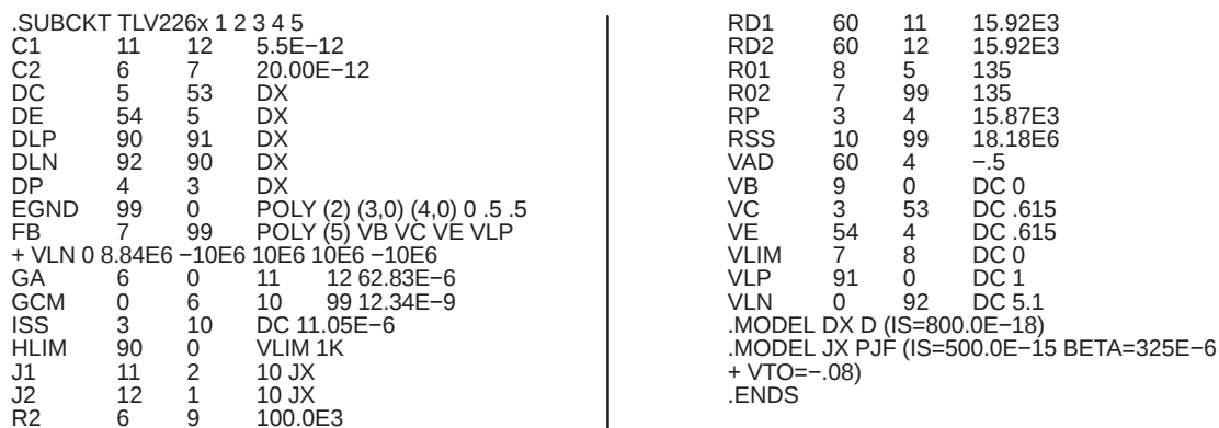
Figure 62. Boyle Macromodel and Subcircuit
