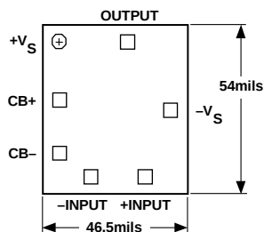
Chip Layout
