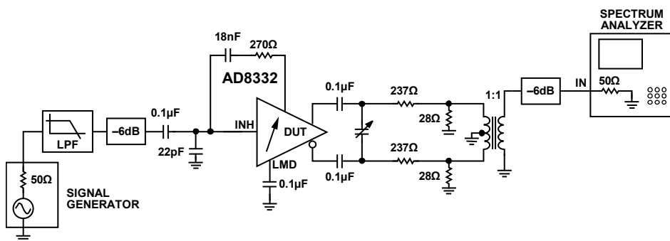
Figure 64. Test Circuit—Harmonic Distortion vs. Load Capacitance
