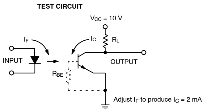
Figure 11. Switching Time Test Circuit and Waveforms
