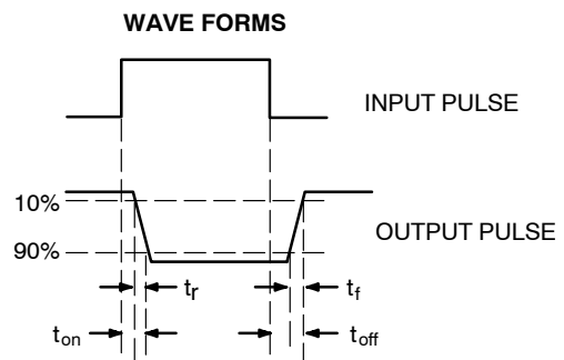
Figure 11. Switching Time Test Circuit and Waveforms
