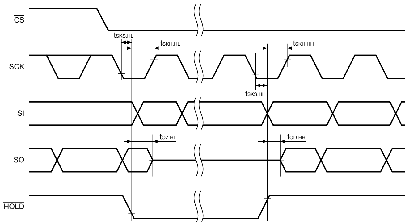
Figure 4 Hold Timing
