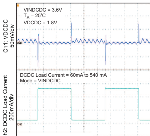
Figure 29. Load Transient Response (DC-DC PWM Mode)
