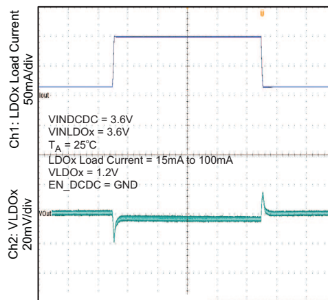
Figure 30. Load Transient Response (LDOx)
